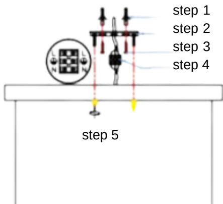
Installation Diagram
